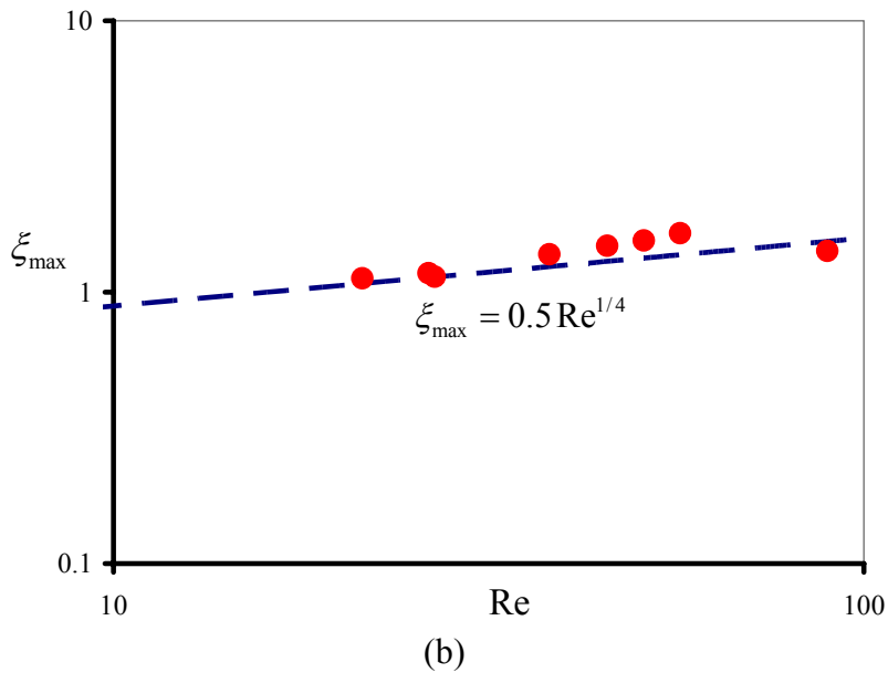
Figure 30: (a) Comparison of LBM simulation results (●) with (a) experiments and correlation of Scheller (---, \Delta ), Asai ( \square ) and correlation of Pasandideh-Fard ( \diamond ). (b) Comparison of LBM (●) with the analytical solution of Pasandideh-Fard (---).
