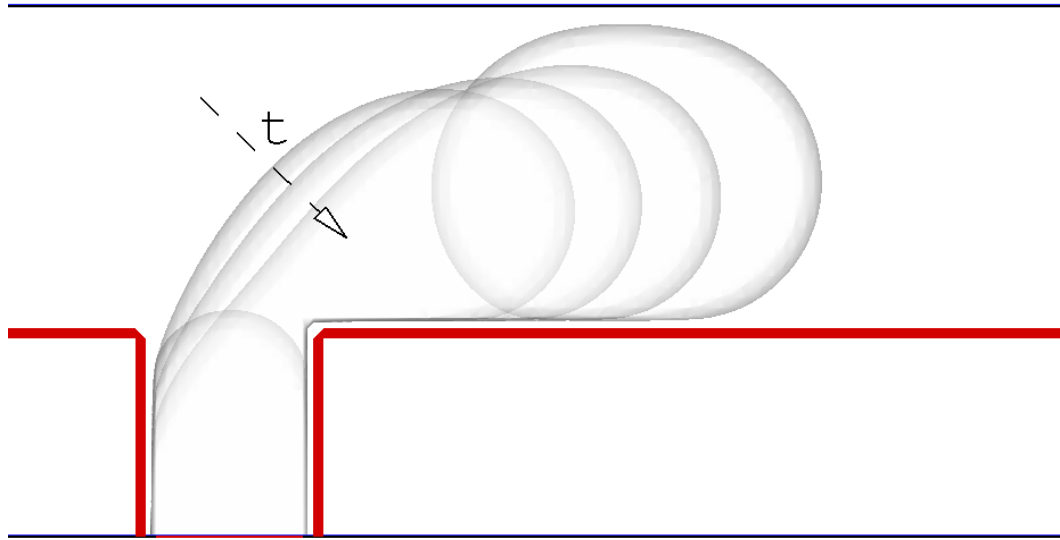
Figure 37: Formation of a plug for Ca=0.0028 and \Lambda = 1/2 using lattice Boltzmann simulations. It can be observed that the upstream interface moves towards the downstream edge of the dispersed phase channel with time, where the interface is pinched-off eventually.
