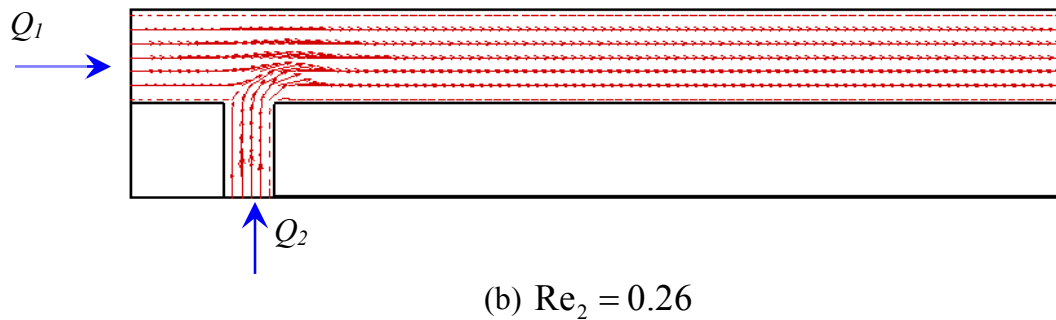
Figure 20: Velocity vectors for different flow rates of the bottom inlet channel. Reynolds number corresponding to Q_1 fixed at Re_1 = 0.16 .
