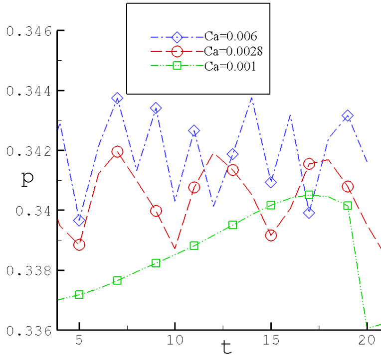
Figure 44: Pressure fluctuation measured upstream of the T-junction for different Capillary numbers.
