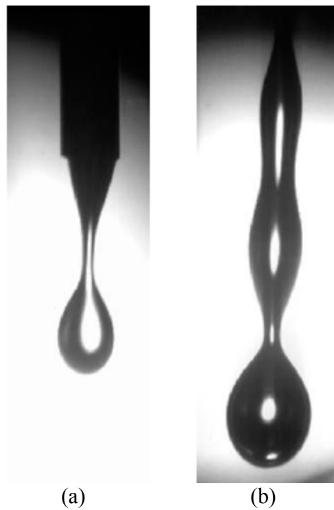
Figure 4: Drop formation in a co-flowing arrangement. The two modes of (a) dripping and (b) jetting are shown (from Cramer et al (2004)).
