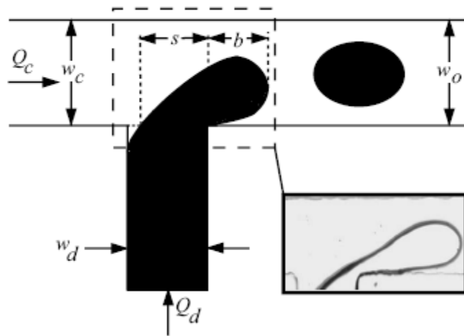
Figure 9: Schematic diagram showing the expanding droplet in the main channel, and (inset) experimental image of the droplet expansion (after Christopher et al (2008)).
